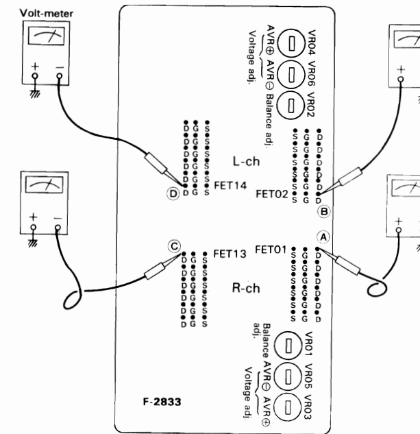
Fig. 3-1 F-2833 MC Head Amp Circuit Board (Component side)
