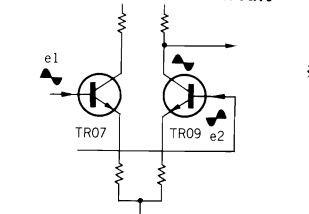
Fig. 2-6 Voltage Differential Circuit
