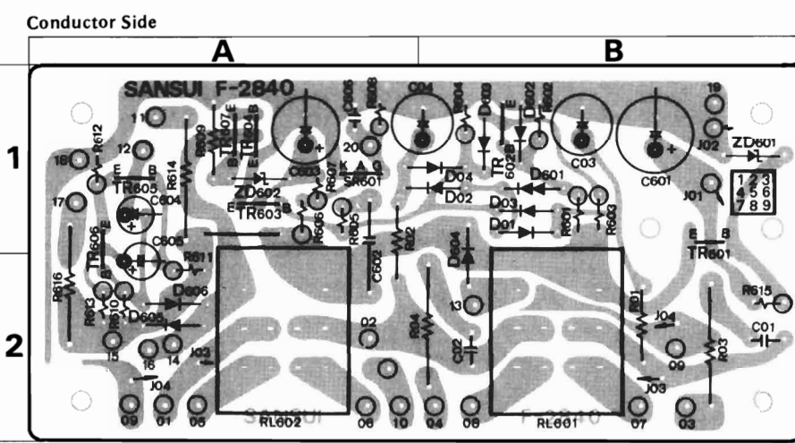
4-5. F-2840 Protector Circuit Board (Stock No. 7596631)
