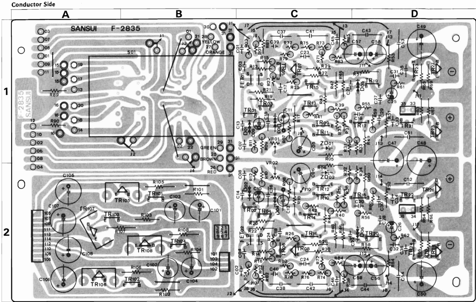
4-3. F-2835 Equalizer Amp Circuit Board (Stock No. 7551331)
