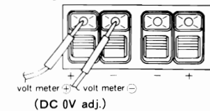
Fig. 3-3 SPEAKER TERMINAL
