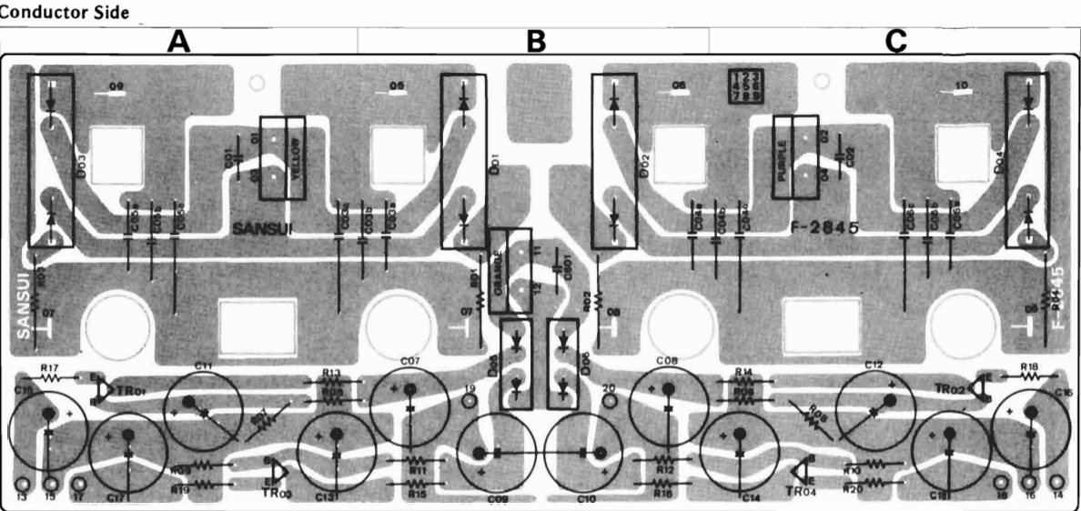
4-4. F-2845 Power Supply Circuit Board for power amp section (Stock No. 7503011)
