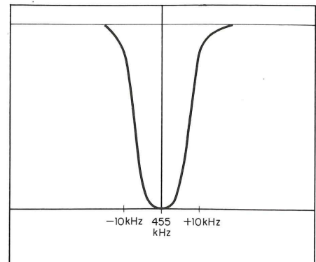
AM IF WAVE FORM
