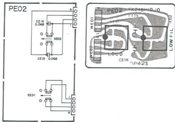
12.10 Low Filter Loud. Assembly (PE02) Schematic Diagram and Component Locations
