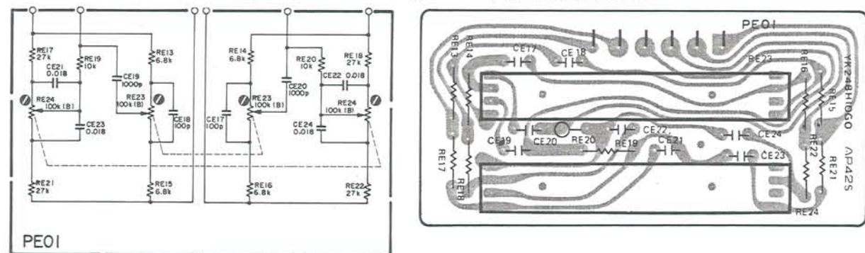
12.11 Tone Volume Assembly (PE01) Schematic Diagram and Component Locations
