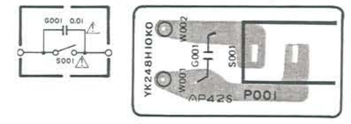
12.6 Power Switch Assembly (P001) Schematic Diagram and Component Locations
