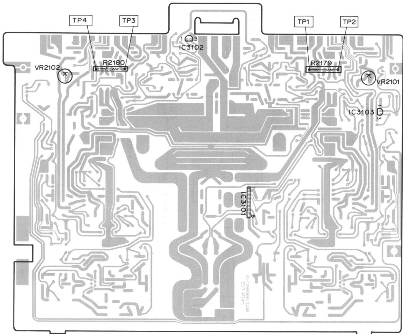
Figure 12 Main P.C. Board (Components Side)
