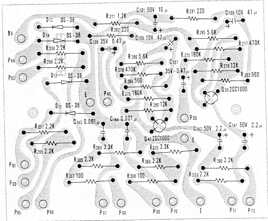
PB938 BOARD
