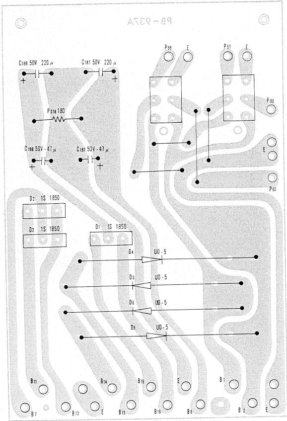
PB937A BOARD
