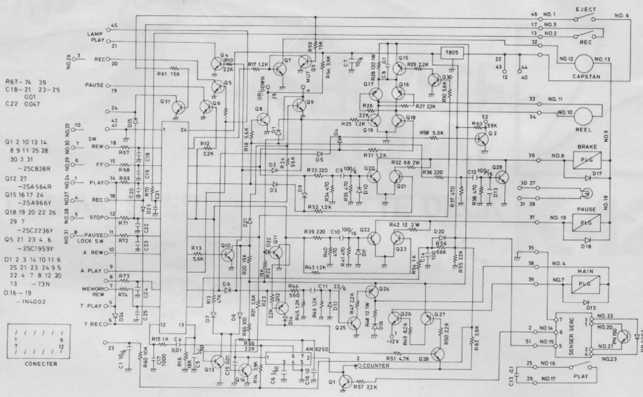
K-12 CONTROL CIRCUIT
