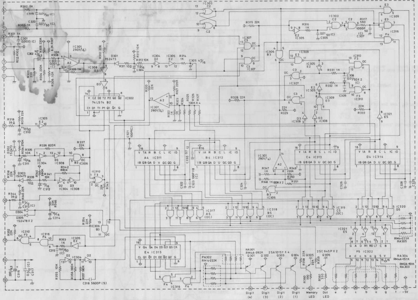
K-12 DIGITAL PCB CIRCUIT
