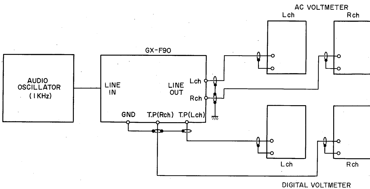
Fig. 28 Instrument Connection
