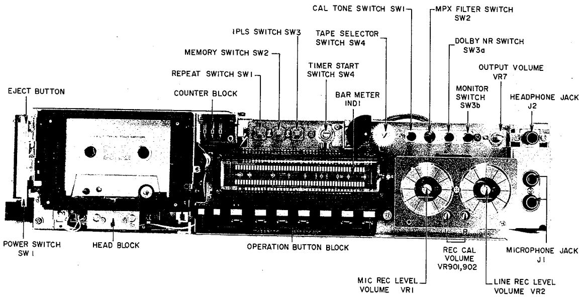
Fig. 2 Front View
