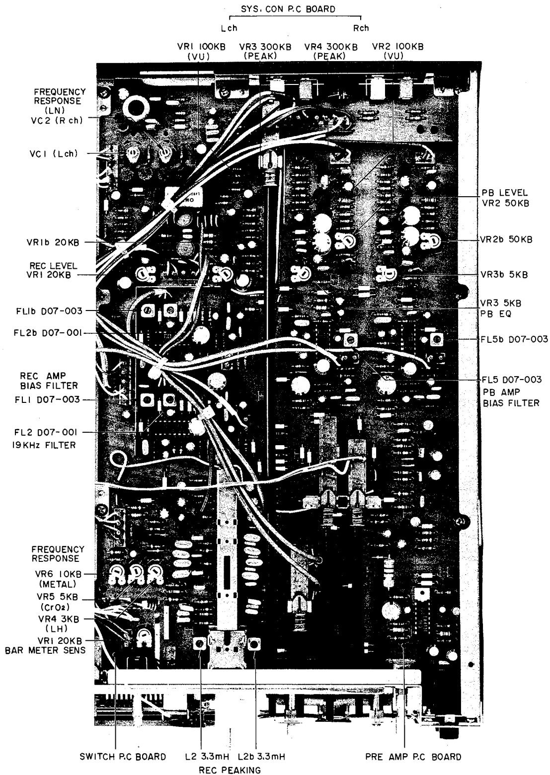
Fig. 24 Amplifier Adjustment Point
