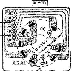
SOCKET P.C BOARD CU-5032C
