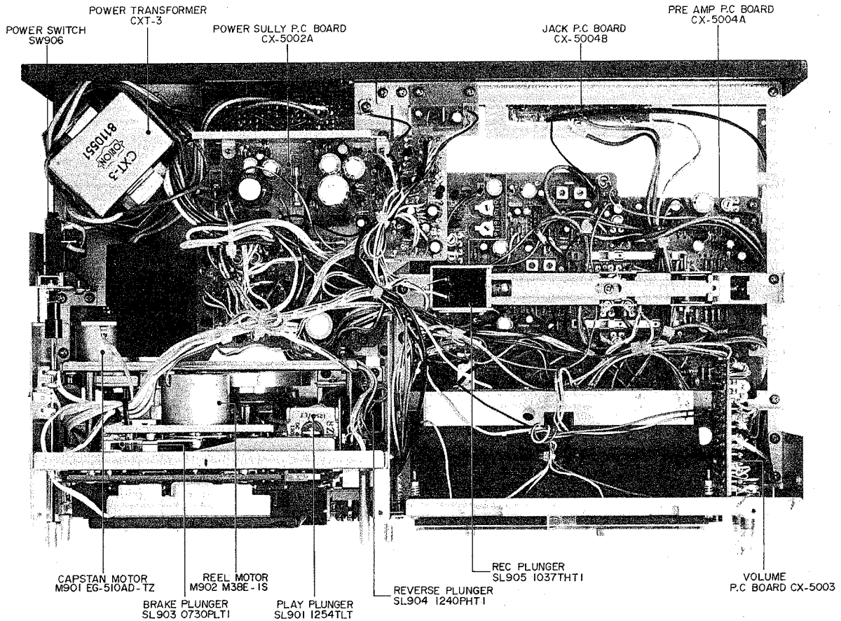
Fig. 3 Top View
