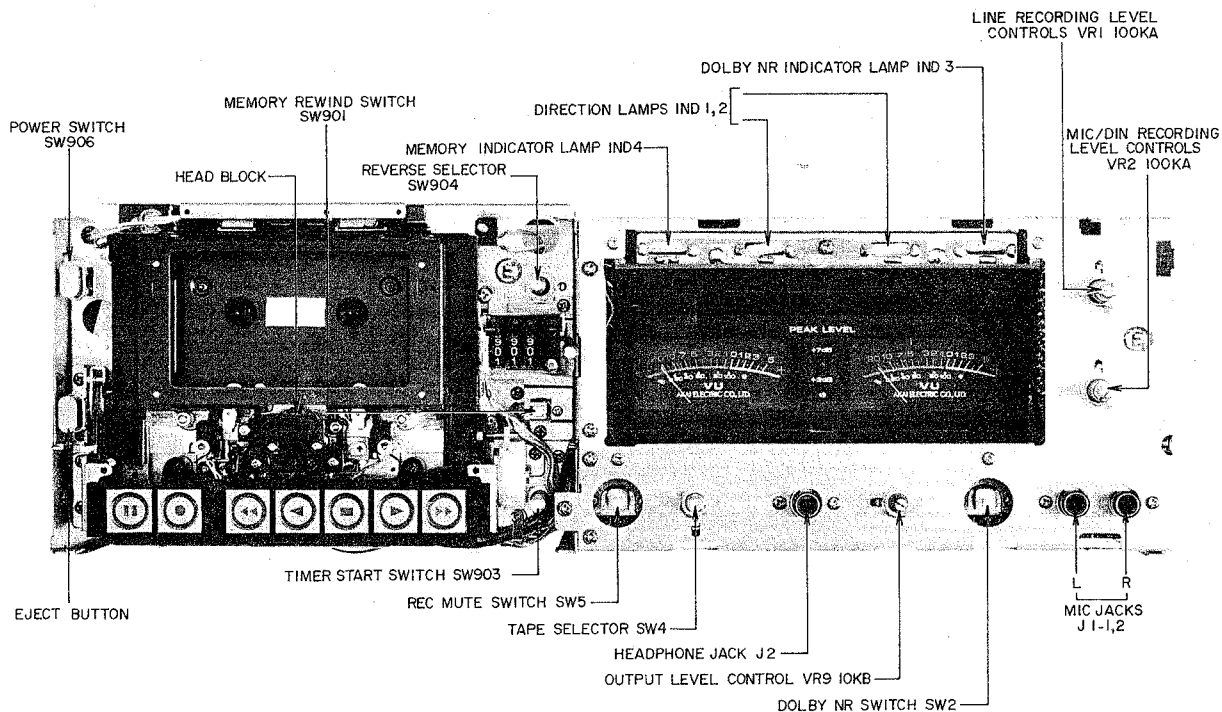
Fig. 2 Front View
