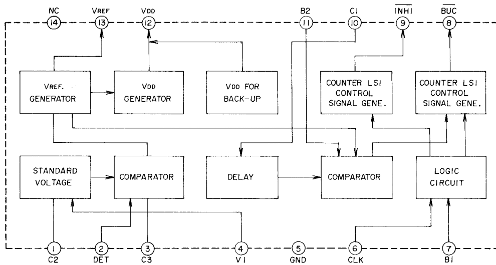
LOGIC CHART
