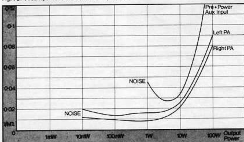
Fig. 14. Intermodulation distortion for the E202
