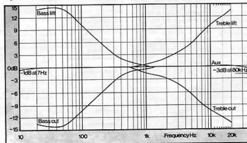
Fig 12. Preamp response and tone controls
