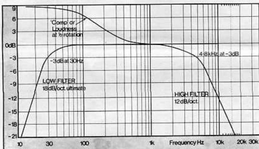
Fig. 13. Preamp filter and loudness responses
