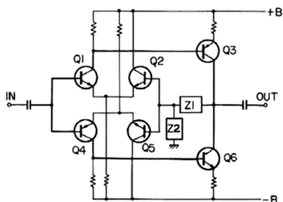
Fig. 1 BASIC CIRCUIT
